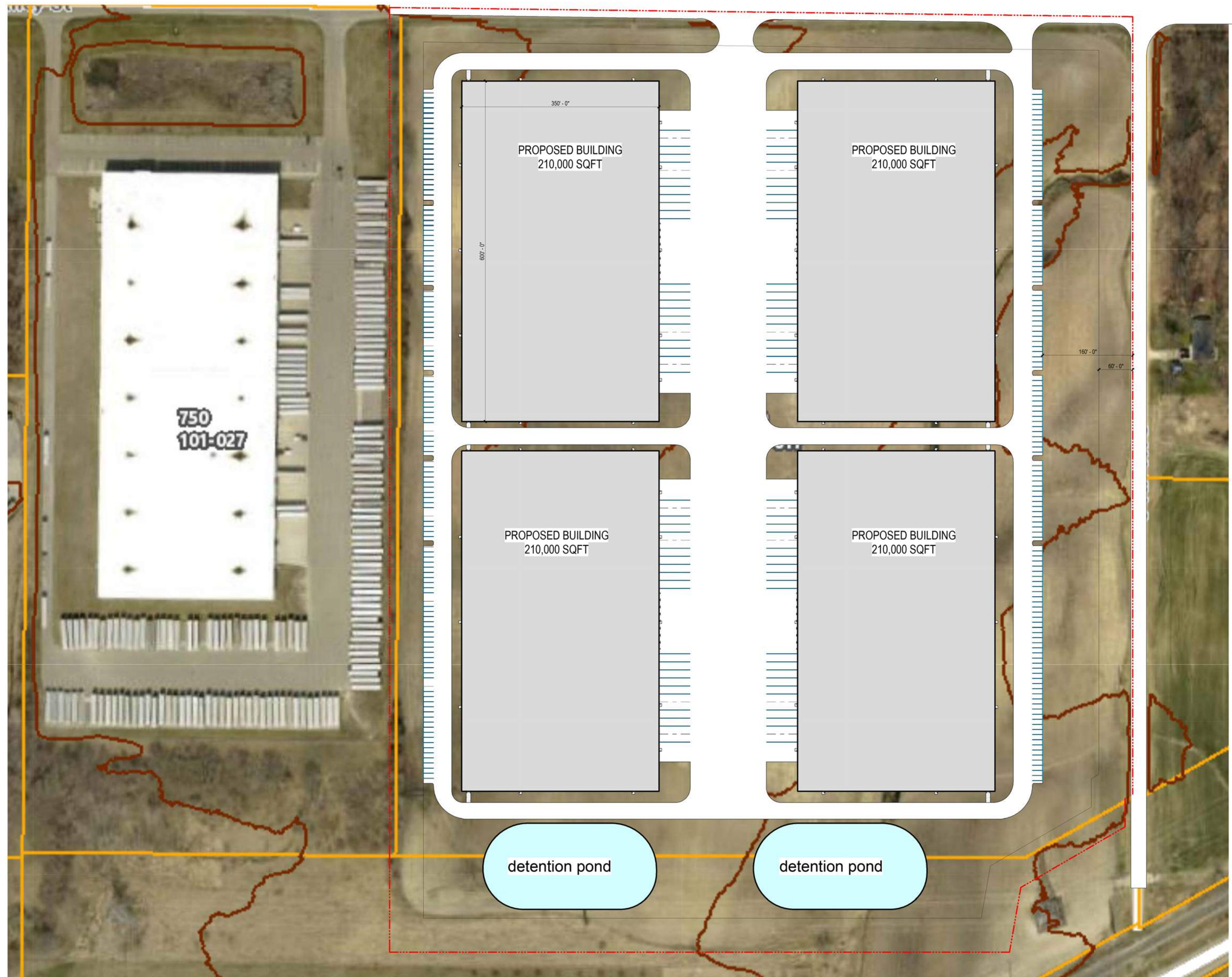
⊕ SITE PLAN (4) BUILDINGS
